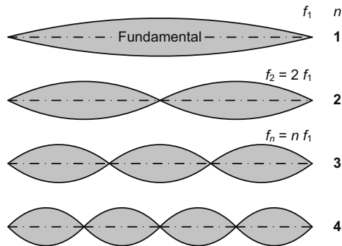
Figure 6.1 Modes of motion in a vibrating string, which are analogous to the modes of motion in a polymer molecule according to the model of Rouse. Modes 1 through 4 are shown. Higher modes involve the coordinated motion of successively shorter segments of the string, as higher Rouse modes represent the coordinated motions of successively smaller groups of submolecules. The analogy is far from perfect, as a molecule is not fixed at its ends
