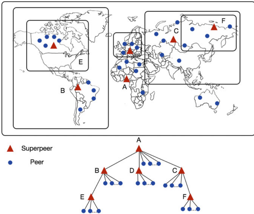
Fig. 2.7 Globase.KOM: division of world projection in multiple non-overlapping zones
