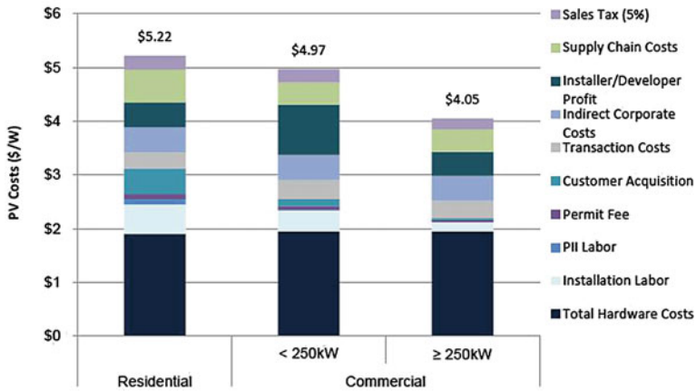
Fig. 2.11 Total US PV system price, by sector and system size ( first half of 2012 ). Opportunities for PV improvements [17]
