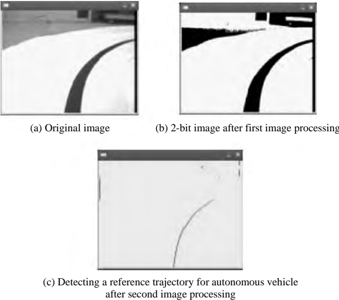
Fig. 6 Image processing based on visual information from camera
