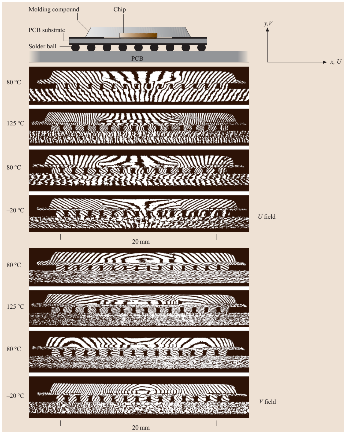
Fig. 1.13 U and V displacement fields for an electronic package subjected to a thermal cycle in an environmental chamber. f = 2400 lines/mm
