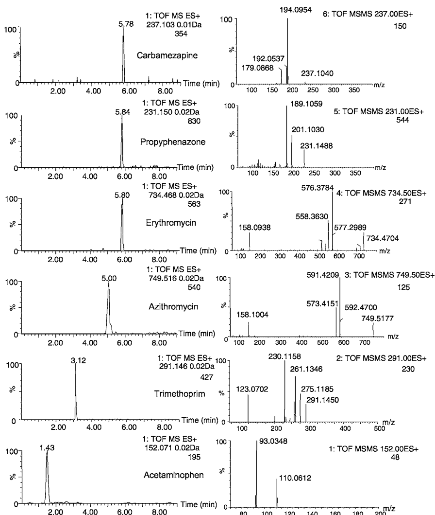
Fig. 4 Confirmation of several pharmaceuticals in an urban wastewater. Left panel : narrow window extracted ion chromatograms (nwXICs) of [M+H]^+ obtained in the TOF mode for m/z 152.071 (acetaminophen), m/z 291.146 (trimethoprim), m/z 749.516 (azithromycin), m/z 734.468 (erythromycin), m/z 231.150 (propyphenazone) and m/z 237.103 (carbamezapine). Right panel : product ion spectra obtained in the Q-TOF mode
