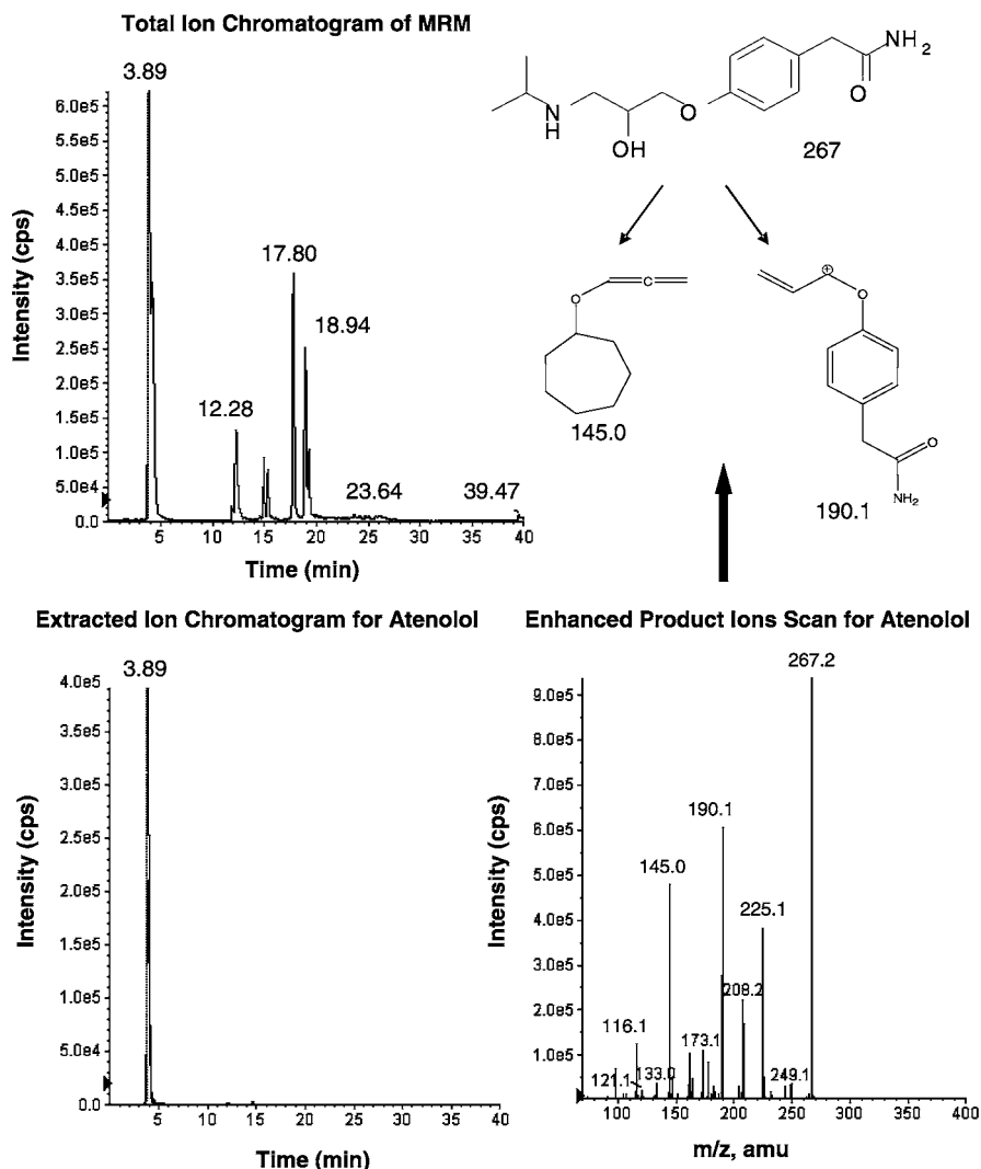
Fig. 5 Information-dependent acquisition (IDA) experiment for the determination of atenolol in an influent wastewater sample
