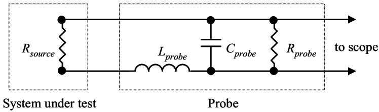
Figure 32: Basic, simplified model of an oscilloscope probe.
