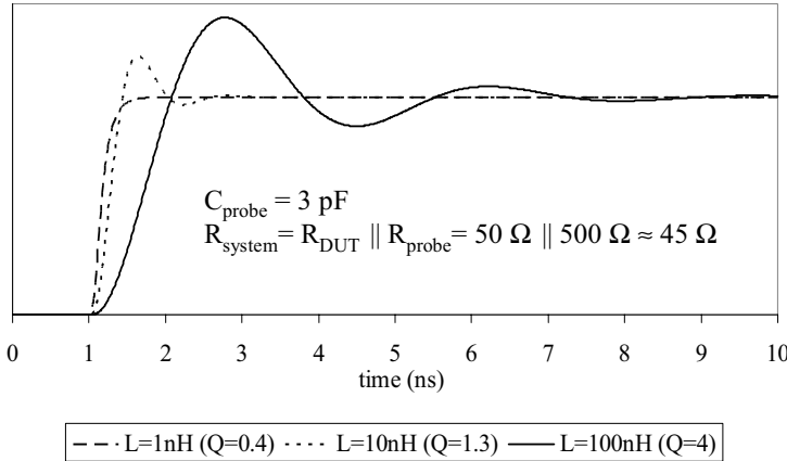
Figure 35: Acquired waveforms for different probe grounding schemes (resulting in different probe inductances), for a passive 500 Ω probe attached to a 50 Ω driver.
