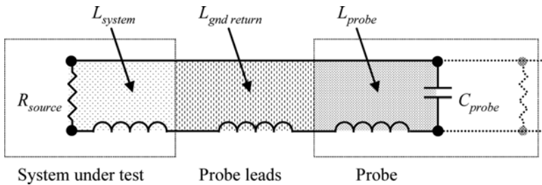
Figure 34: Current loop of system, probe, and ground return path, causing parasitic inductance.
