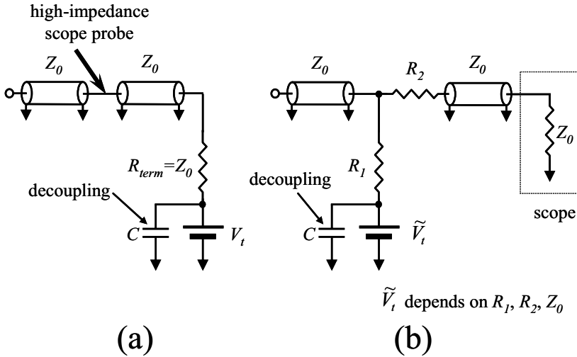
Figure 45: Providing matched termination to a bias level: (a) For a high-impedance probe. (b) Thevenin-equivalent termination for a matched impedance probe that by itself terminated to ground.
