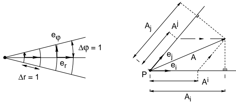
Fig. 2.3. Left: polar co-ordinates and the base vectors e_r and e_\varphi . Right: interpretation of the contravariant and covariant representation of a vector A .
