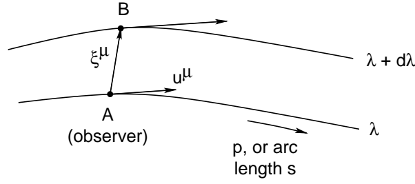
Fig. 2.9. The geodesic deviation.
