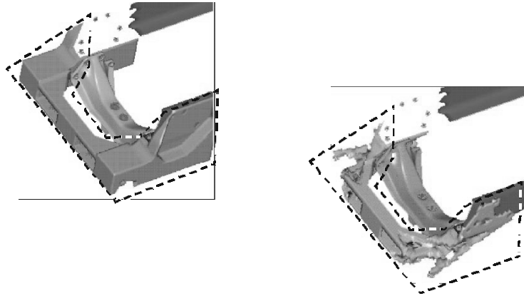
Figure 4: Topology Optimization
