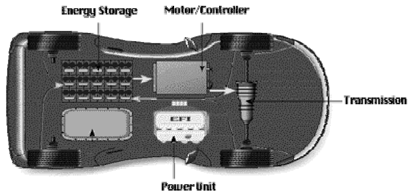
Parallel Vehicles
