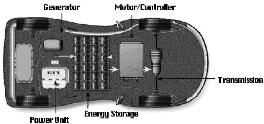
Series Vehicles
