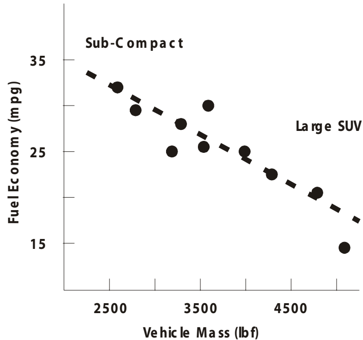
Figure 7: Fuel Economy
